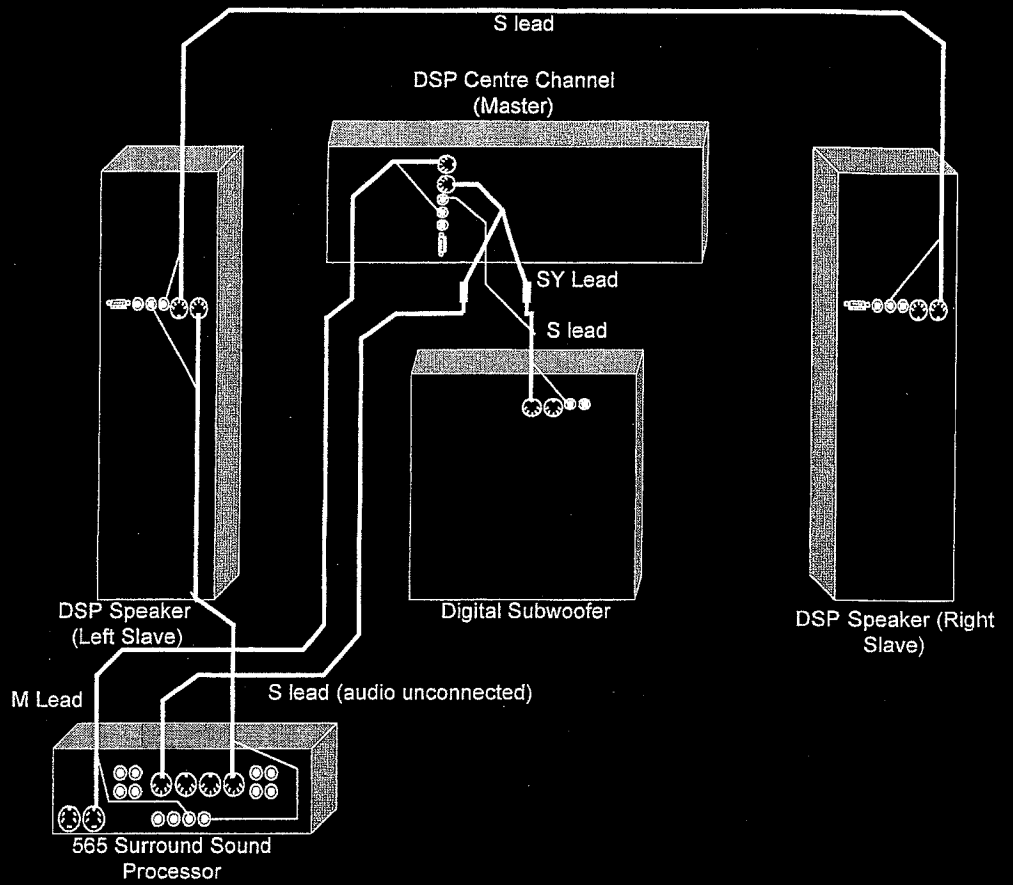
Figure 1: A typical centre/5.1 subwoofer installation
