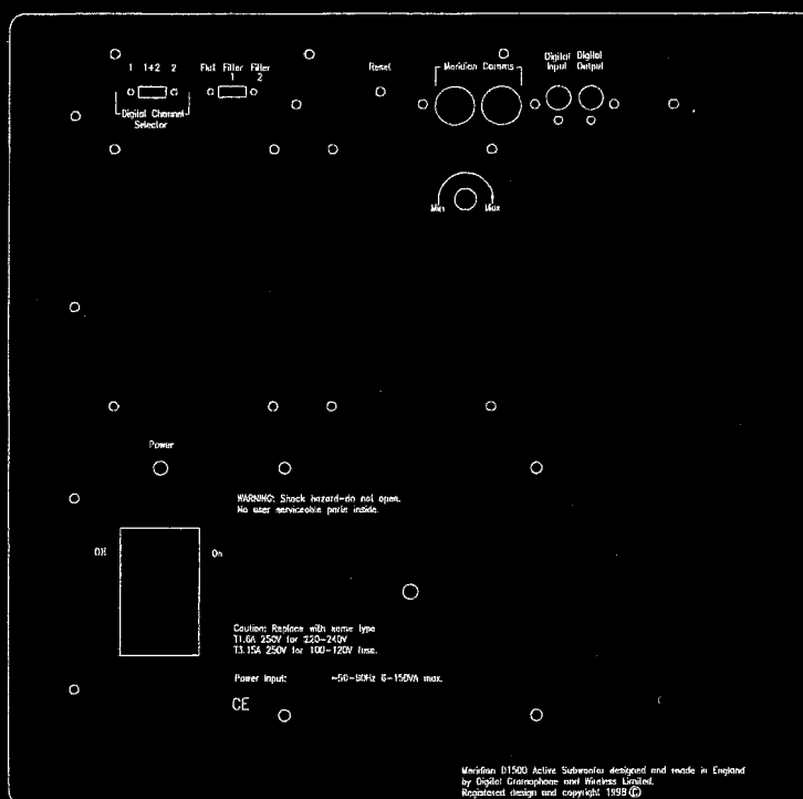
Figure 7 Rear Panel
